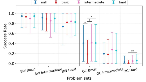
Figure 5: Success rate for Blocksworld (BW) and Overcooked (OC) domains when generated without visual data ( null ), with visual data of basic problems ( basic ), with visual data of intermediate problems ( intermediate ), and with visual data of hard problems ( hard ). They are then tested with PANDA solver with basic, intermediate, and hard problem sets.
