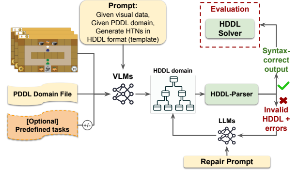
Figure 1: Structure of Vision2HTN Framework.
